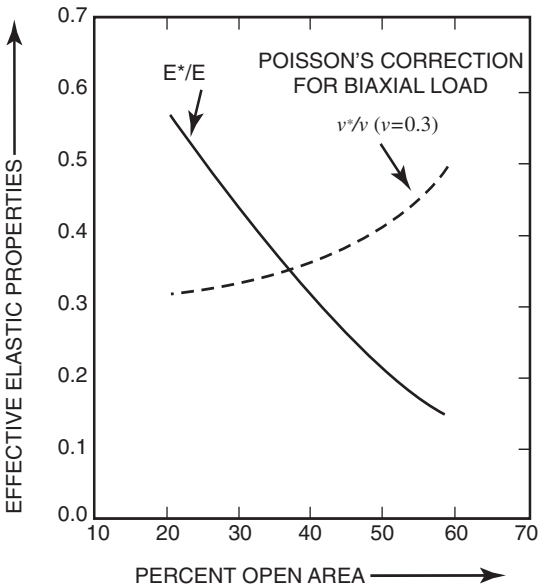
Figure 4: Effective Elastic Modulus, E^* , and Poisson's Ratio, \nu^* , vs. Percent Open Area
