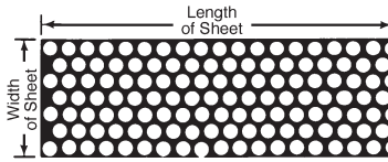
Figure 1: Standard 60° Staggered Pattern Showing Length and Width Orientations
